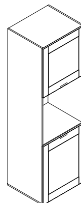
MSTCI616S MSTCI616D 600x515x1960
