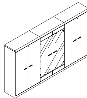
WD212C 2514x380x1400
